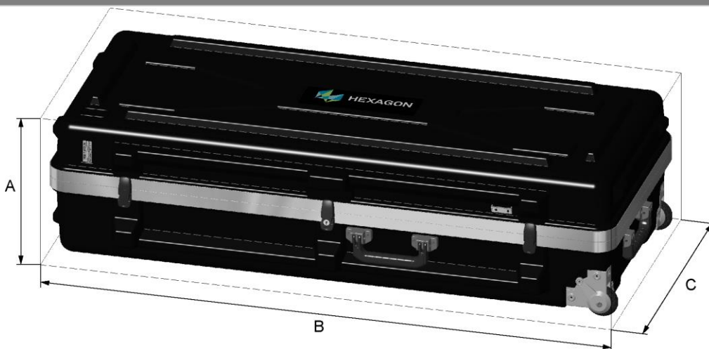
Fig. 43: Travel case dimensions
