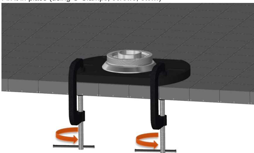
Fig. 26 : Mounting plate installation
