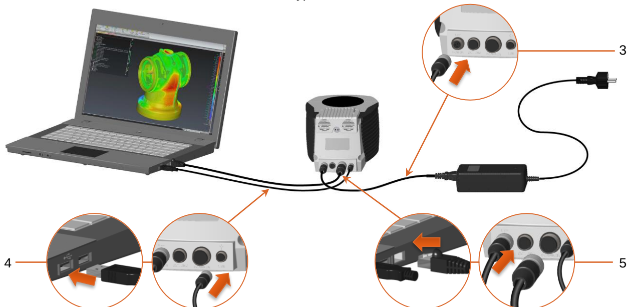
Fig. 35 : HP-L-20.8 connection
